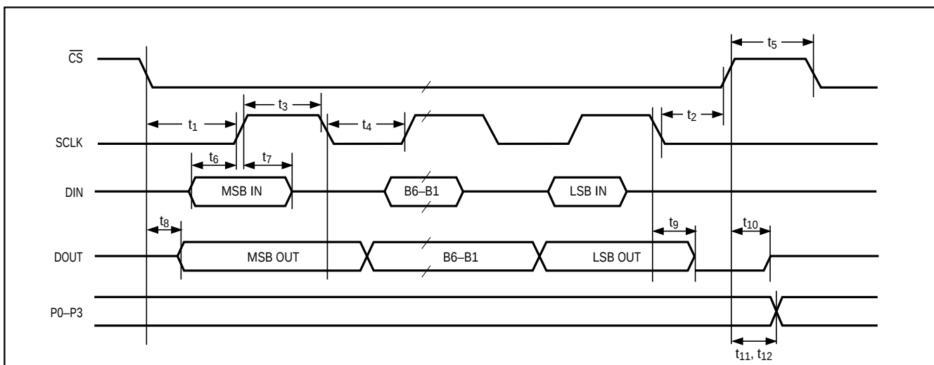
Figure 2. Serial-Mode Timing
