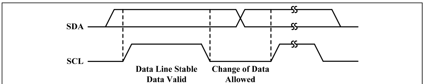
Figure 3 Bit transfer
