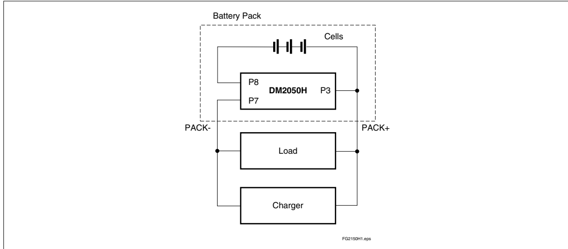
Figure 1. Module Connection Diagram
