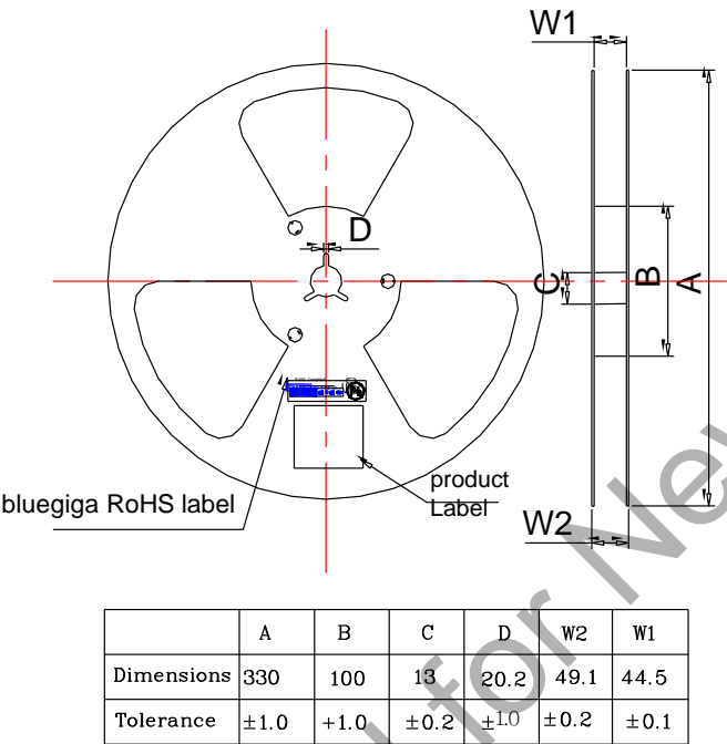
Figure 31: Reel information
