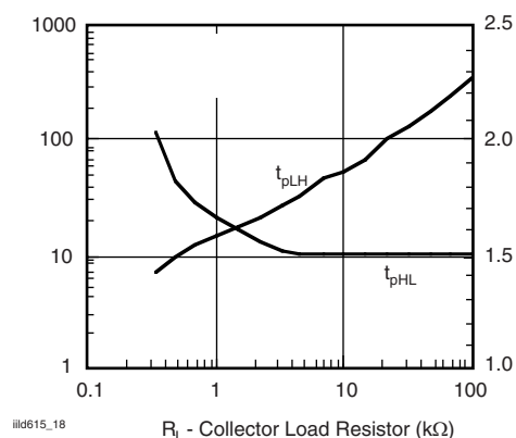
Fig. 19 - -2, -3, Propagation Delay vs. Collector Load Resistor
