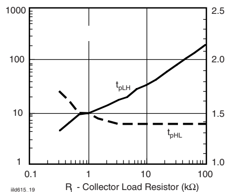
Fig. 20 - -4, Propagation Delay vs. Collector Load Resistor
