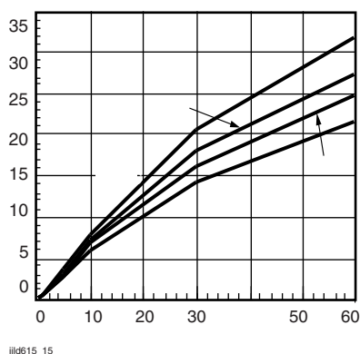
Fig. 16 - Collector Emitter Current vs. Temperature and LED Current
