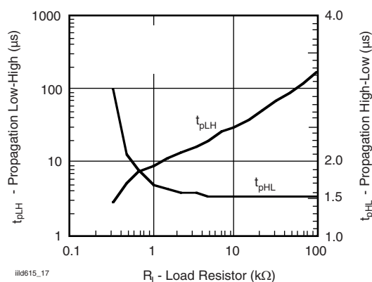
Fig. 18 - -1, Propagation Delay vs. Collector Load Resistor
