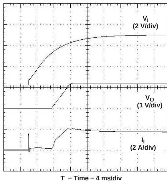
Figure 20. Power-Up Waveform
