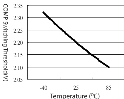
COMP switching Threshold vs. Temperature
