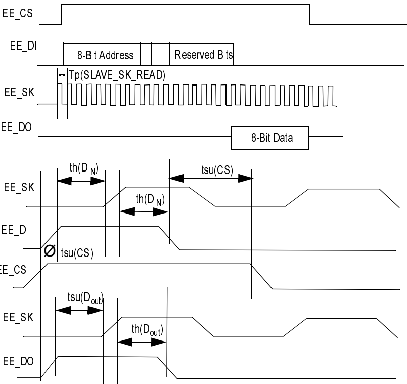
Figure 15. Read Slave Timing
