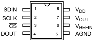
8 Lead SOIC (Jedec, 0.150")
