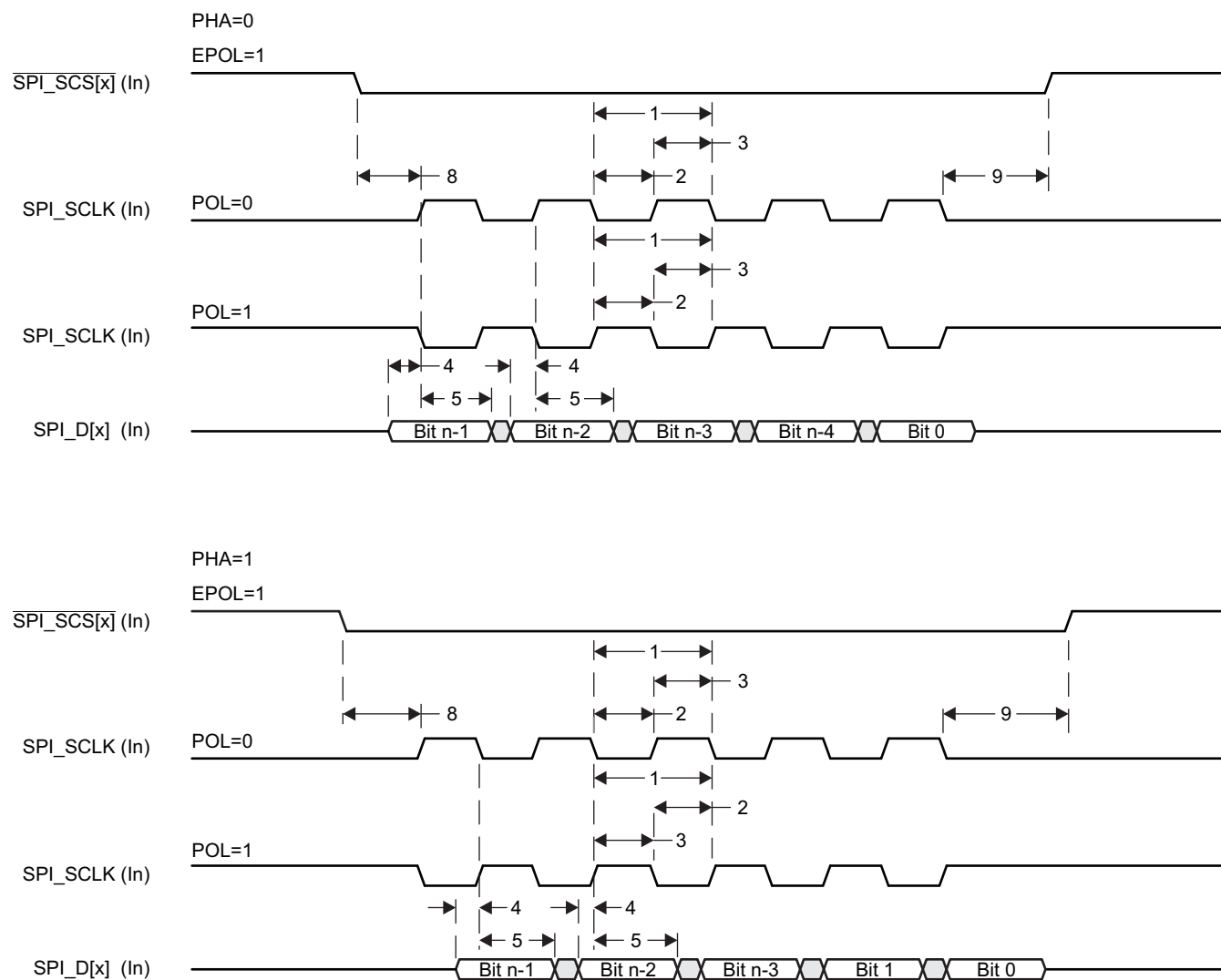
Figure 9-92. SPI Slave Mode Receive Timing
