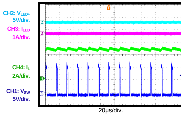
LED+ Short to VSS Steady State
