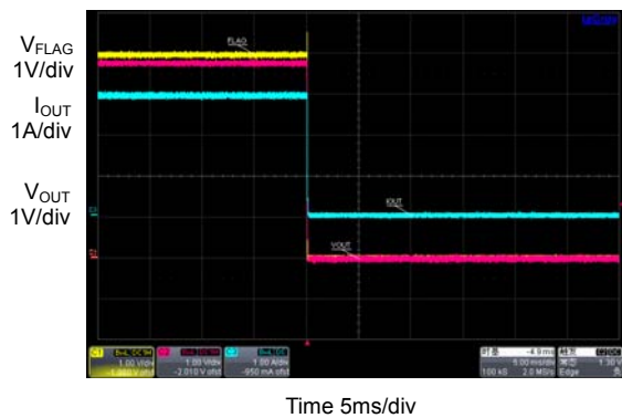
Figure 30. FLAG Response during Over Temperature ( T_A=125\text{ }^{\circ}C )
