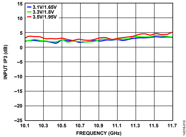
Figure 10. Input IP3 vs. Frequency Various Supply Voltages
