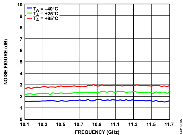
Figure 5. Noise Figure vs. Frequency for Various Temperatures
