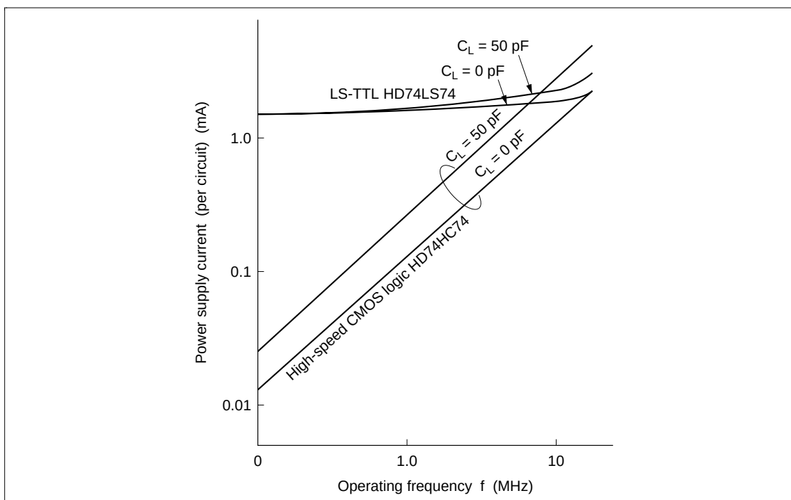
Figure 13 Operating Frequency vs Power Supply Current
