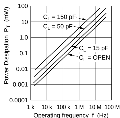
Figure 8 Power Dissipation VS. Operating Frequency
