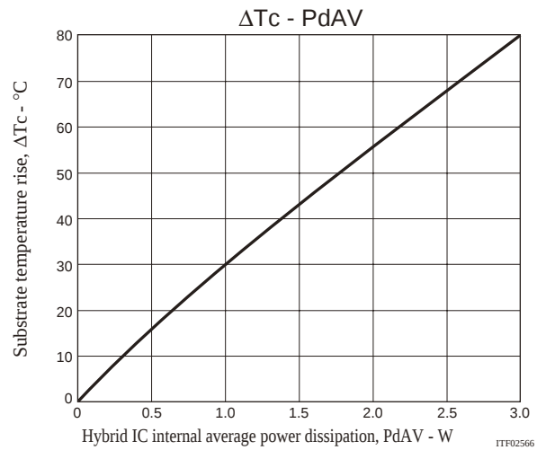
Substrate temperature rise, \Delta T_c (no heat sink) - Internal average power dissipation, P_{dAV}
