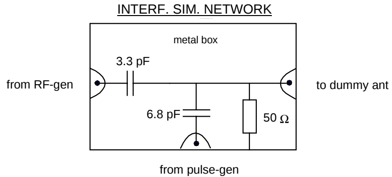
Fig. 8.11 ISN schematics
