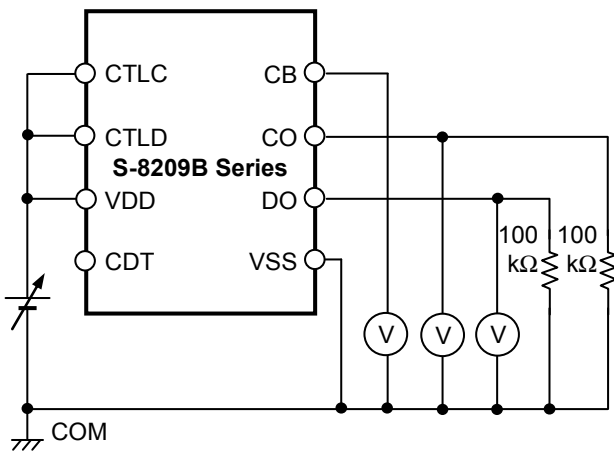
Figure 7 Test circuit 1
