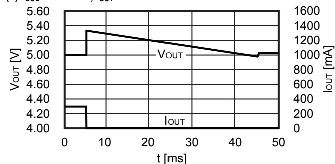
(4) f_{OSC} = 600\text{ kHz} , I_{OUT} = 300\text{ mA} \rightarrow 0.1\text{ mA} S-8366ABBBA
