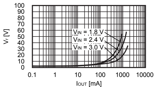
Condition 6 S-8365ABBBA ( V_{OUT(S)} = 3.3 V)
