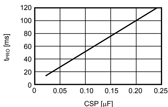
Figure 18 CSP vs. t_{PRO}
