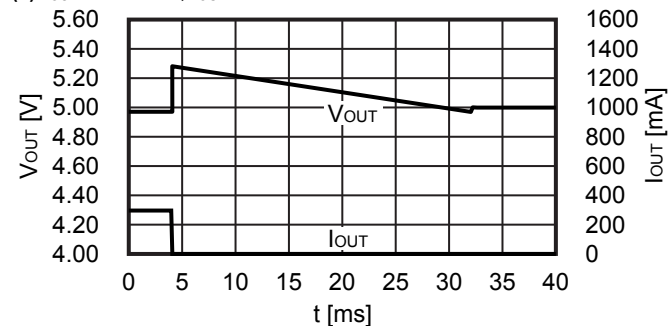
(2) f_{OSC} = 1.2\text{ MHz} , I_{OUT} = 300\text{ mA} \rightarrow 0.1\text{ mA} S-8366AABBA
