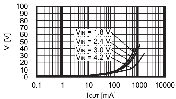
Condition 10 S-8365ABBBA ( V_{OUT(S)} = 5.0 \text{ V} )
