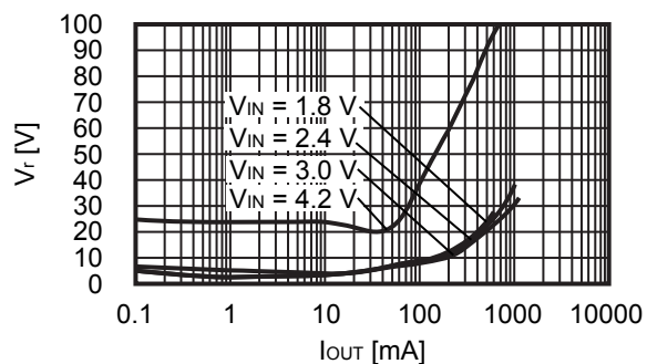
Condition 12 S-8366ABBBA ( V_{OUT(S)} = 5.0 \text{ V} )
