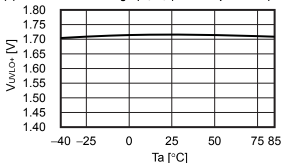
(9) UVLO release voltage ( V_{UVLO+} ) vs. Temperature ( T_a )
