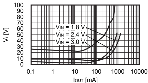
Condition 8 S-8366ABBBA ( V_{OUT(S)} = 3.3 V)
