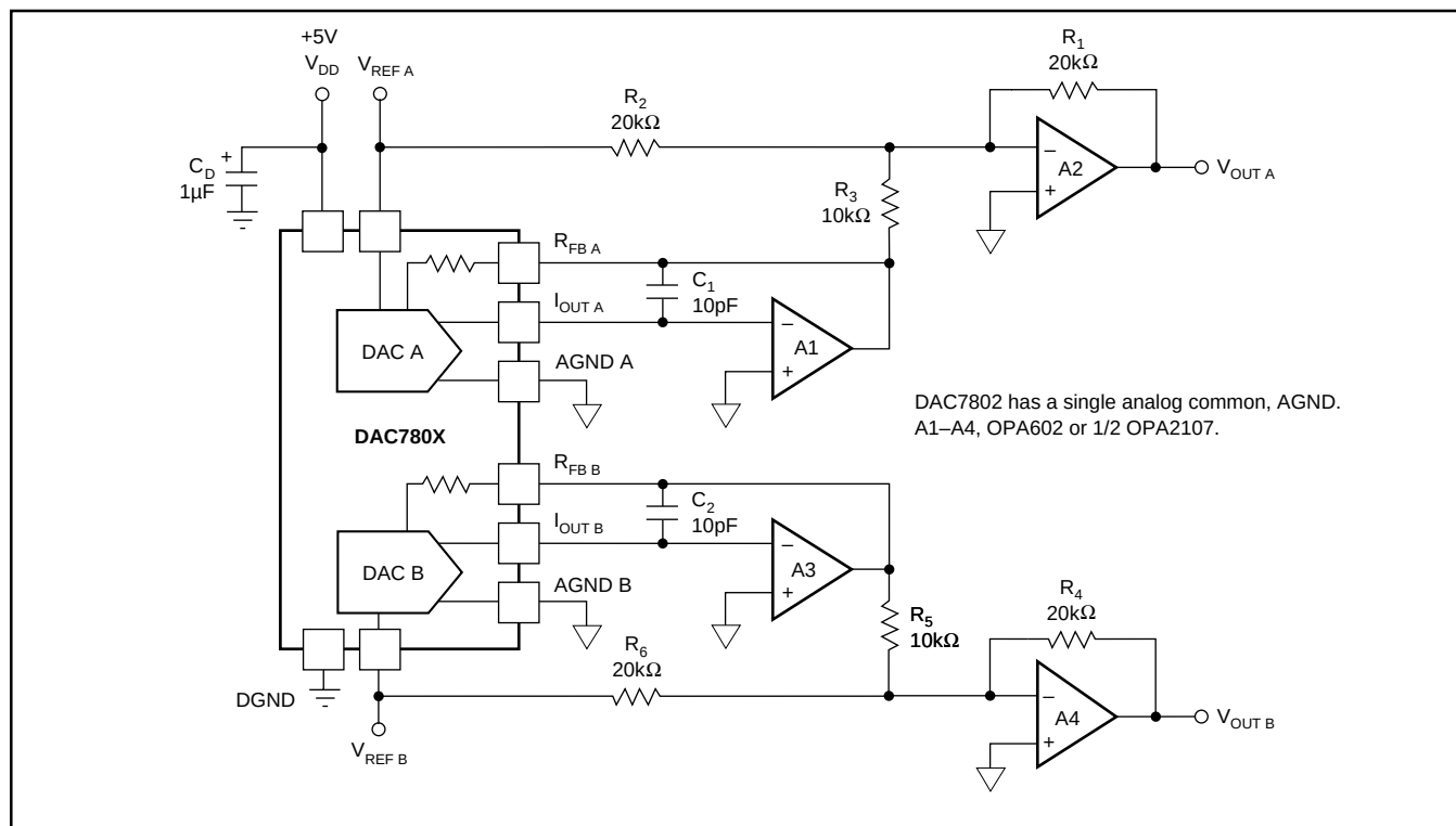
FIGURE 5. Bipolar Configuration.
