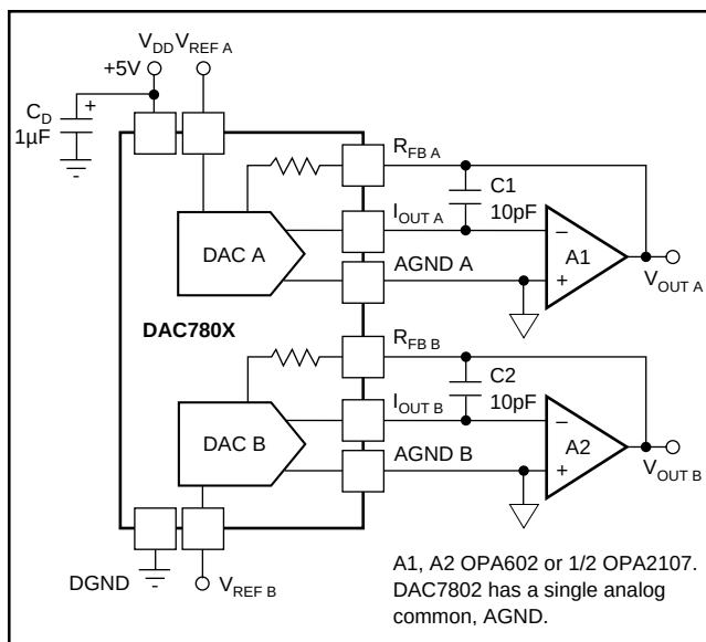
FIGURE 3. Unipolar Configuration.
