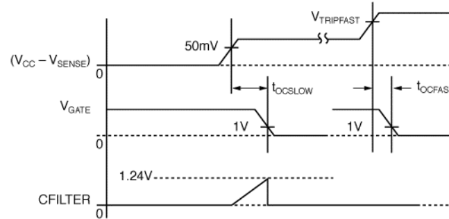
Figure 1. Current-Limit Response
