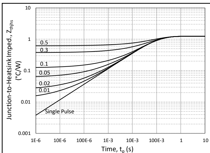
Figure 17. MOSFET Junction to Case Transient Thermal Impedance, Z_{thjcs} ( ^\circ\text{C/W} )
