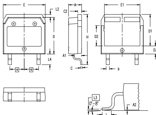
L019a TO-268 AA (D 3 PAK HV)
