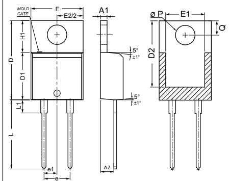
L005b TO-220AC
