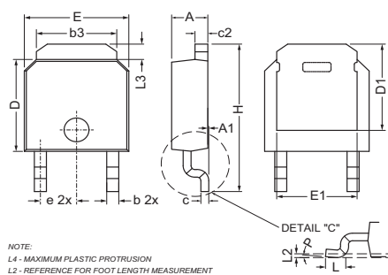
L004a TO-252
