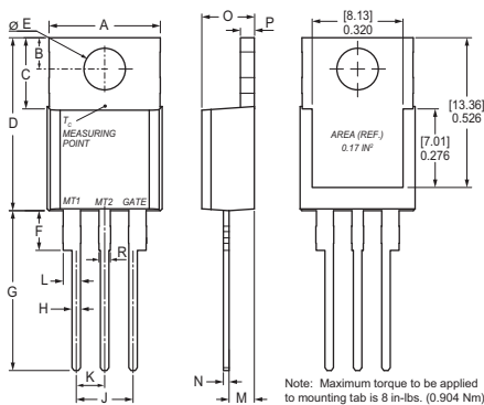
L005c TO-220AB (ISO)
