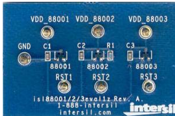
FIGURE 14. ISL88001/2/3EVAL1Z PHOTOGRAPH
