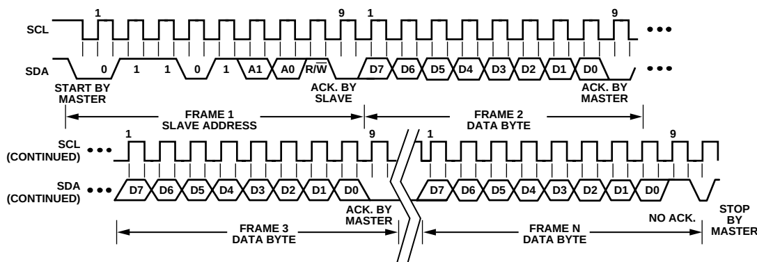
Figure 32. General SMBus Read Timing Diagram
