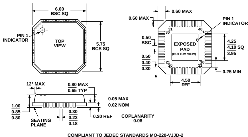
Figure 43. 40-Lead Lead Frame Chip Scale Package [LFCSP] (CP-40)
