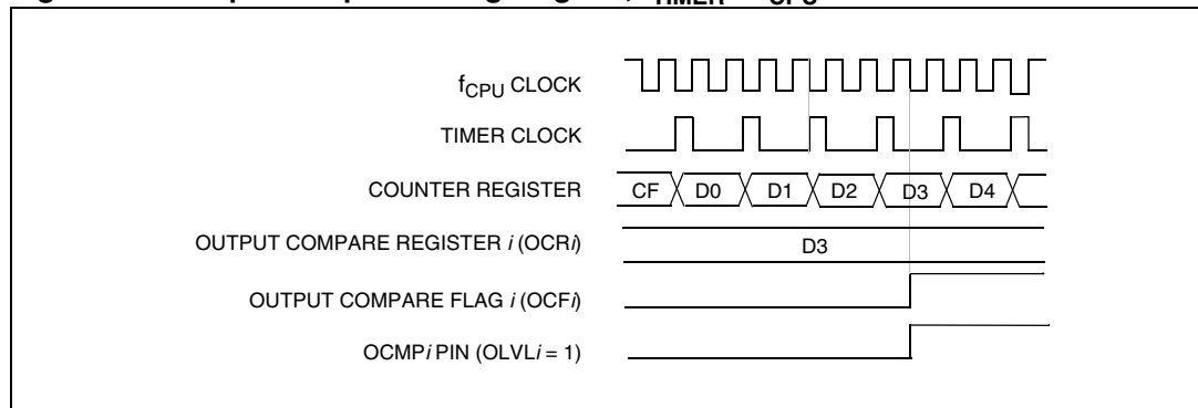
Figure 66. Output compare timing diagram, f_{\text{TIMERB}} = f_{\text{CPU}}/2
