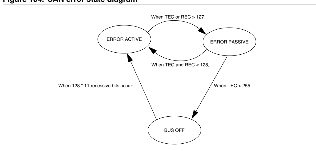
Figure 104. CAN error state diagram
