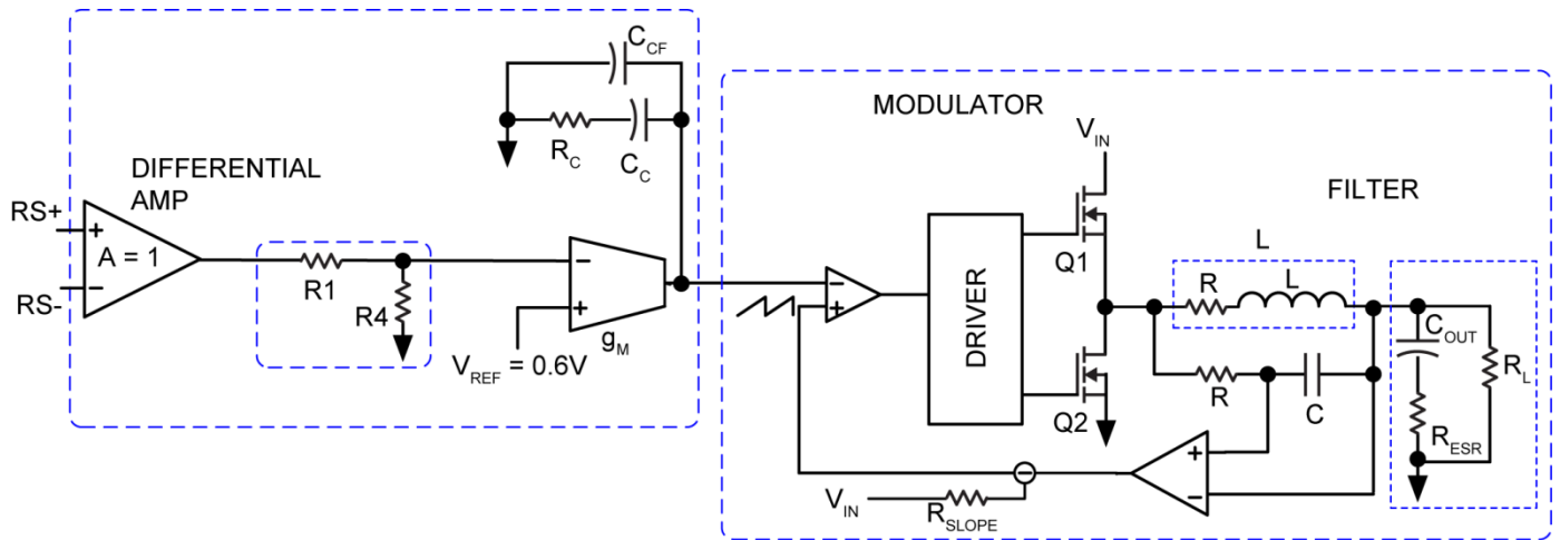
Figure 15. Valley Current Mode Loop Compensation
