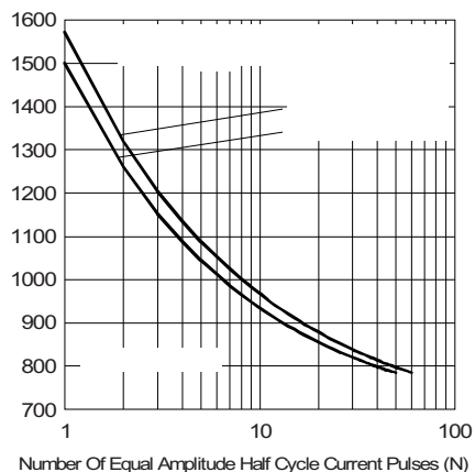
Fig. 21 - Maximum Non-Repetitive Surge Current
