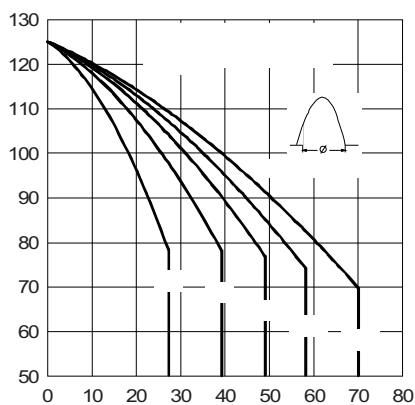
Fig. 9 - Current Ratings Characteristics
