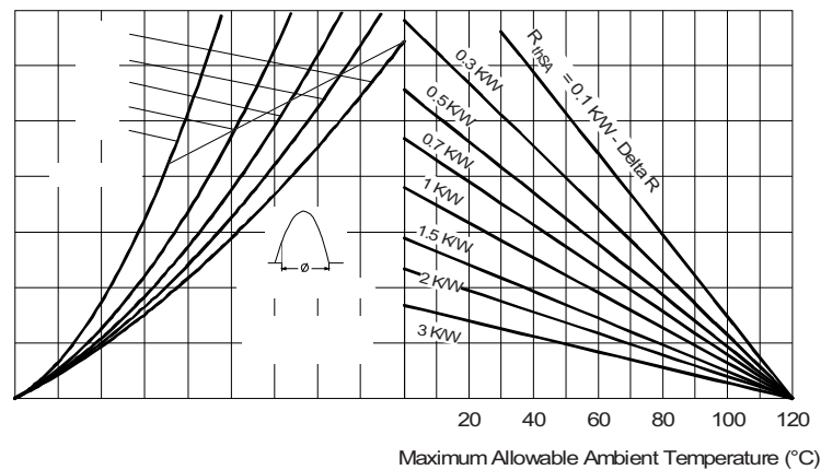
Fig. 19 - On-State Power Loss Characteristics
