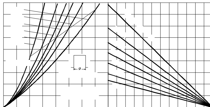
Fig. 20 - On-State Power Loss Characteristics
