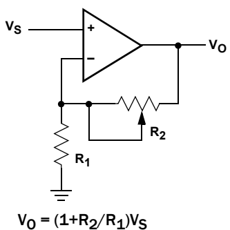
FIGURE 15. NONINVERTING AMPLIFIER
