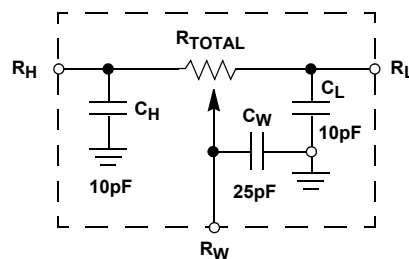
FIGURE 3. CIRCUIT #3 SPICE MACRO MODEL
