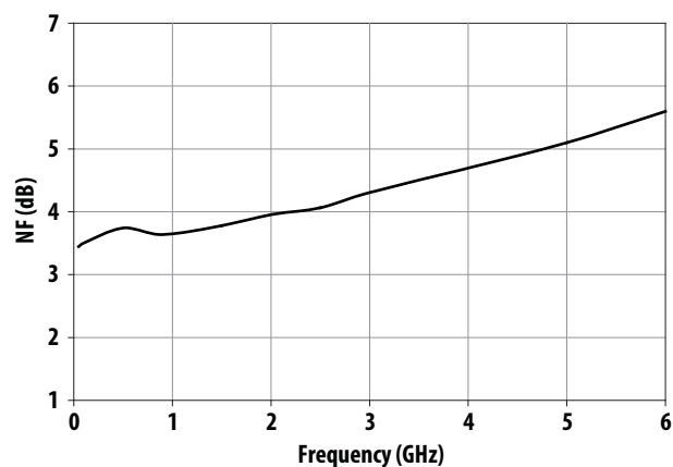
Figure 8. NF vs Frequency at I_d = 45\text{mA}
