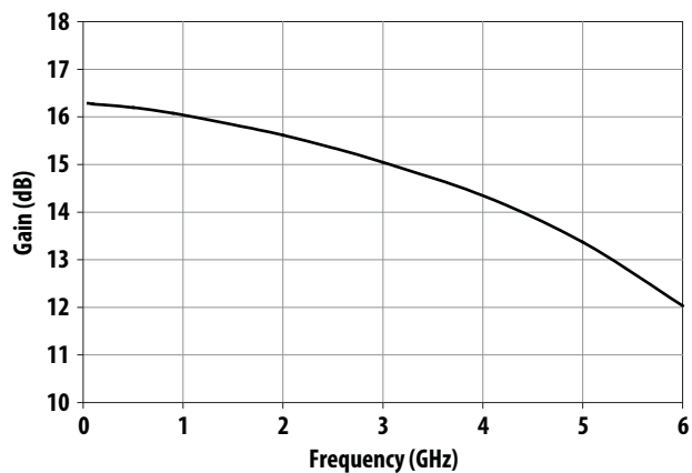
Figure 5. Gain vs Frequency at I_d = 45\text{mA}
