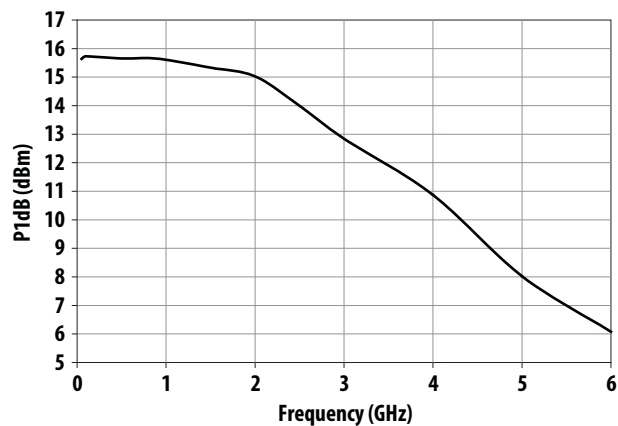
Figure 6. P1dB vs Frequency at I_d = 45\text{mA}
