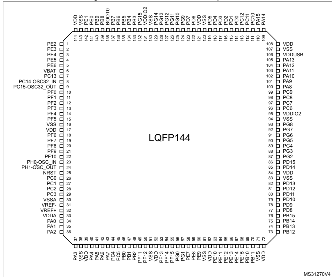
Figure 4. STM32L476Zx LQFP144 pinout (1)
