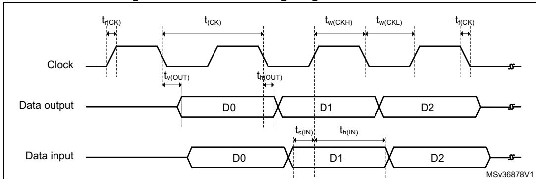
Figure 31. Quad SPI timing diagram - SDR mode
