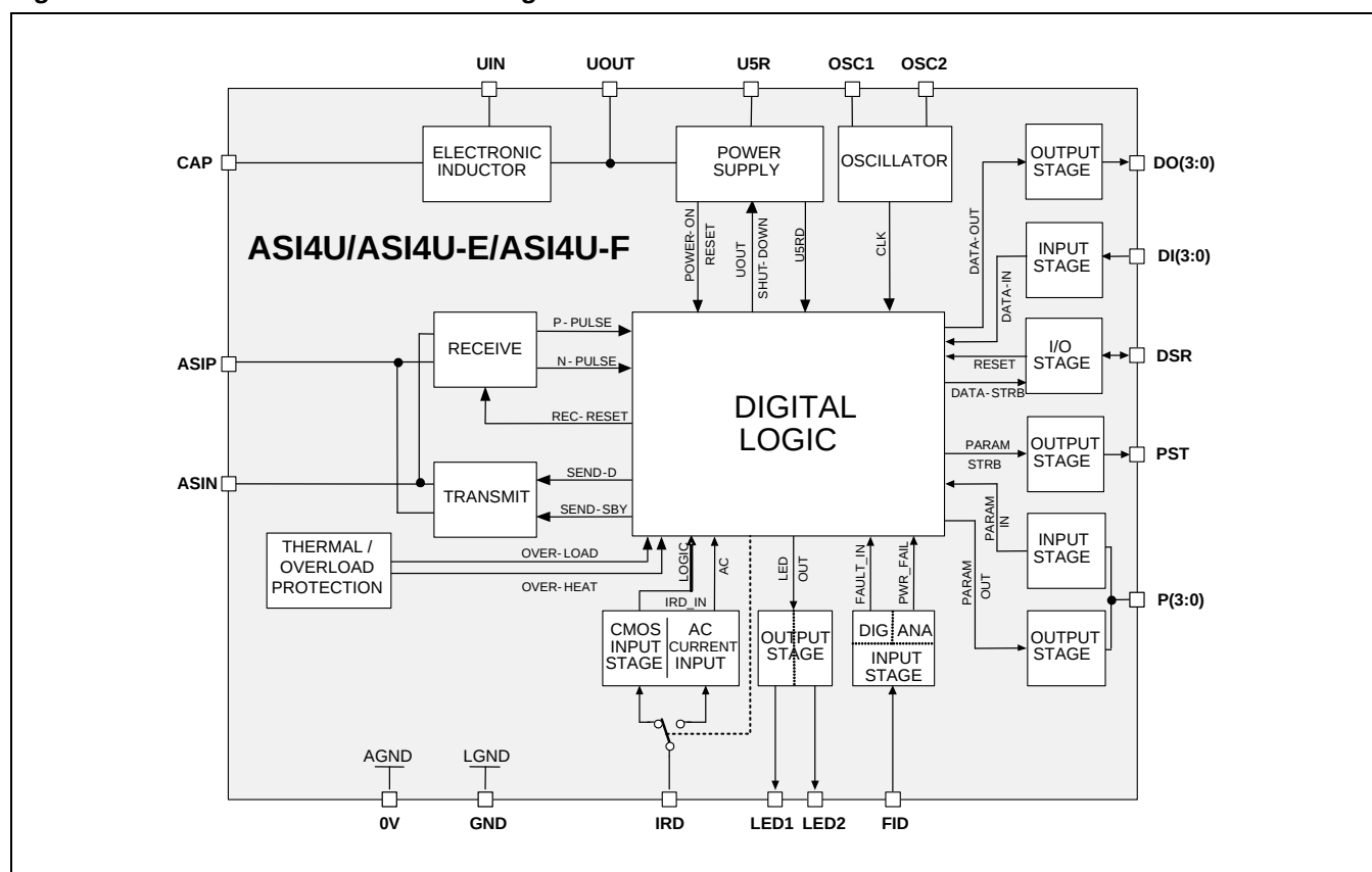
Figure 3.1 ASI4U Functional Block Diagram
