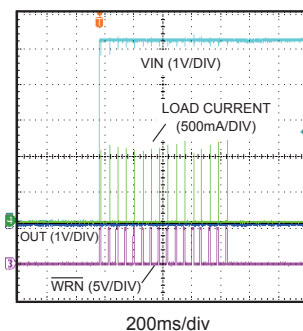
Power-up Waveform when Output is Short-circuit
