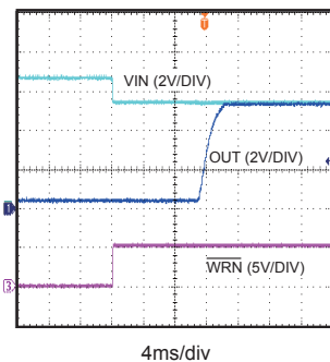
Input Steps From 6.5V to 5.5V Waveform
