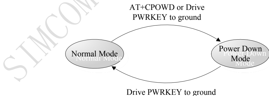
Figure 15: State Transition
