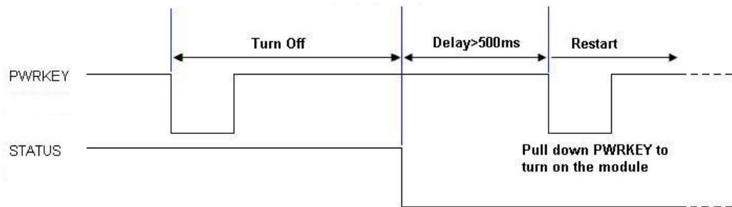
Figure 14: Timing of restart system
