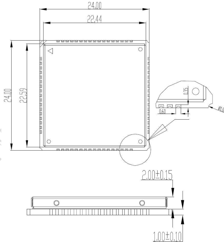
Figure 36: Top and Side Mechanical dimensions of module (Unit: mm)
