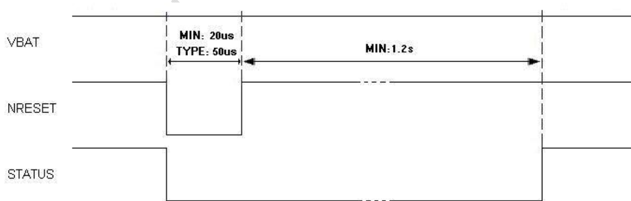
Figure 35: Reset timing
