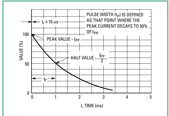
Figure 7. Pulse Waveform
