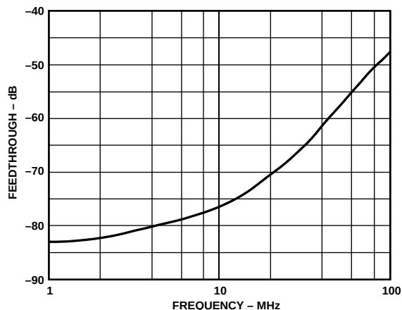
Figure 53. 2:1 Mux OFF Channel Feedthrough vs. Frequency
