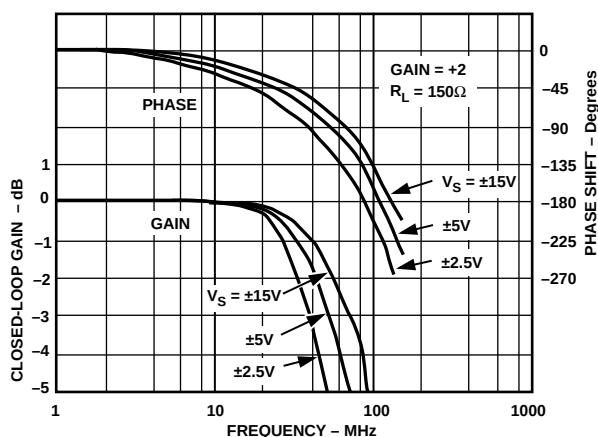
Closed-Loop Gain and Phase vs. Frequency, G = +2 , R_L = 150 \Omega , R_F = 715 \Omega
