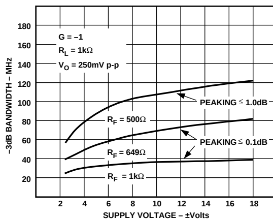
Figure 36. -3 dB Bandwidth vs. Supply Voltage, Gain = -1, R_L = 1 \text{ k}\Omega
