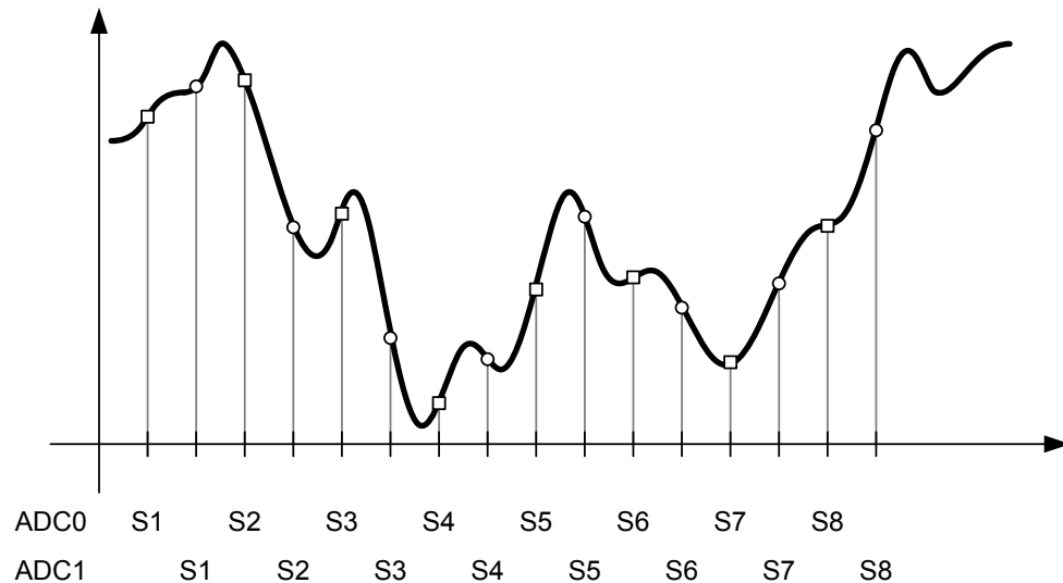
Figure 11-5. Skewed Sampling
