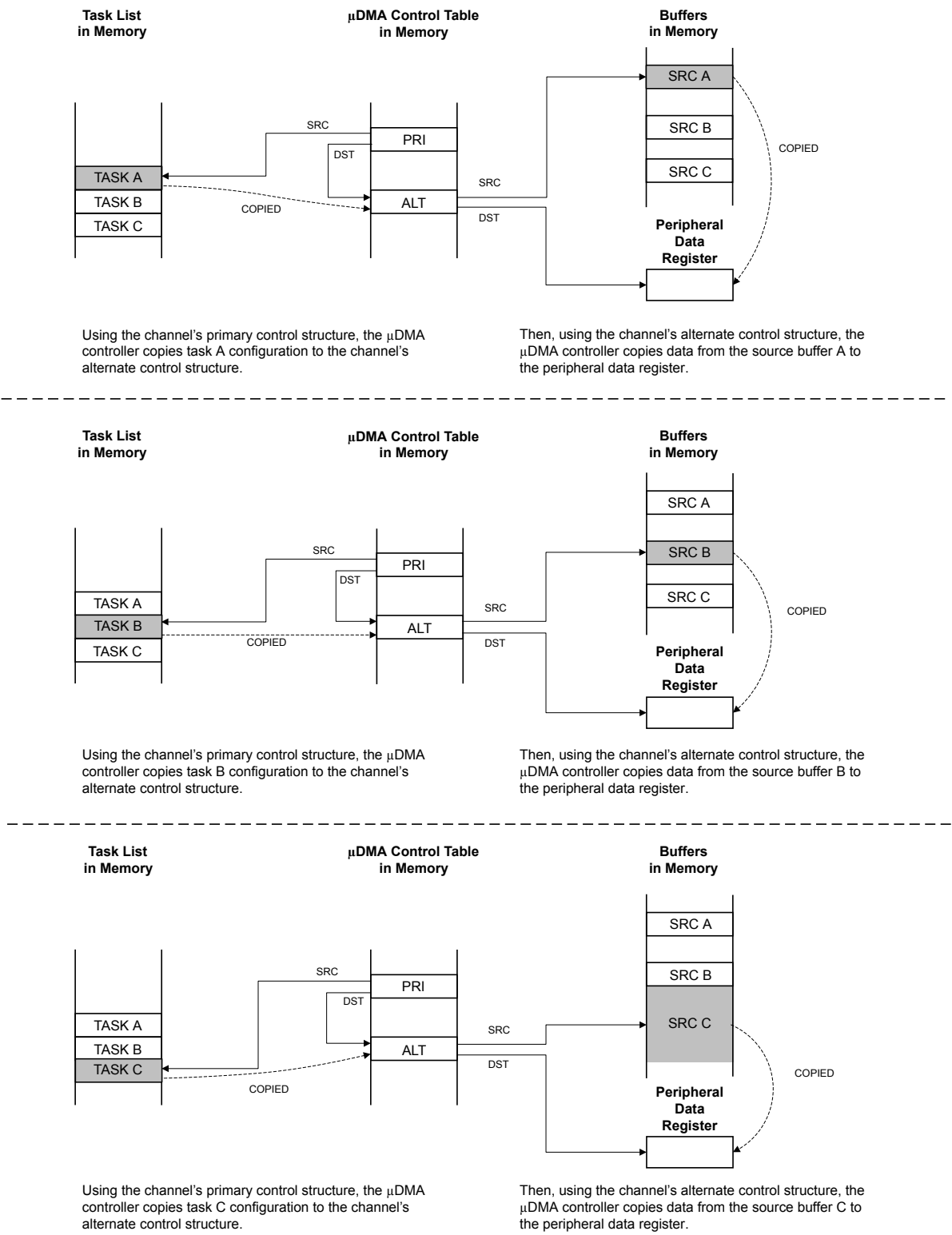
Figure 7-6. Peripheral Scatter-Gather, μDMA Copy Sequence
