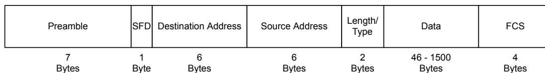
Figure 17-3. Ethernet Frame
