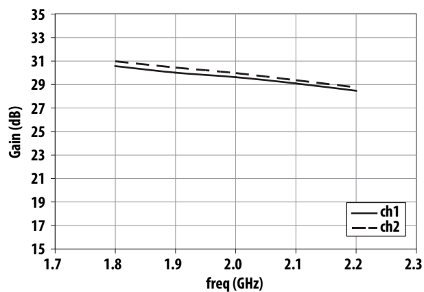
Figure 10. Gain vs Frequency and channel
