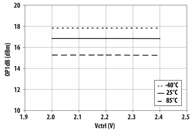
Figure 21. OP1dB vs Vctrl and temperature
