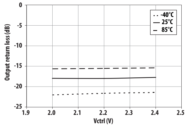
Figure 23. S22 vs Vctrl and temperature
