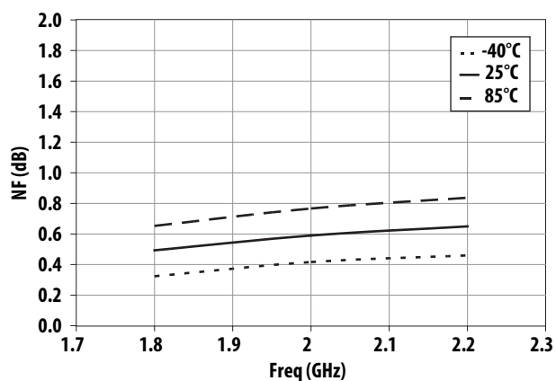
Figure 14. NF vs Frequency and temperature
