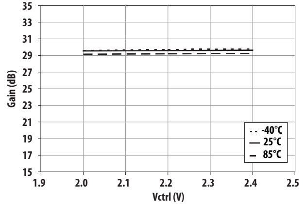
Figure 19. Gain vs Vctrl and temperature
