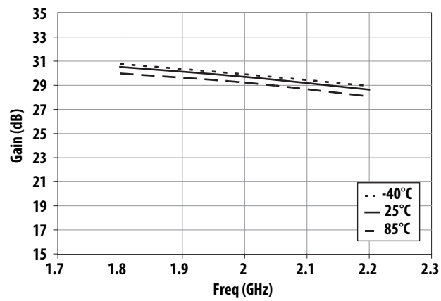
Figure 15. Gain vs Frequency and temperature
