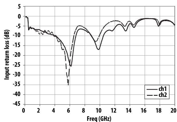
Figure 12. S22 vs Frequency and channel
