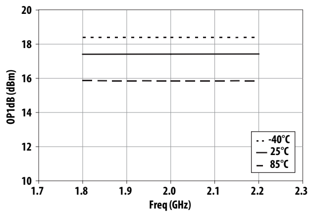
Figure 17. OP1dB vs Frequency and temperature
