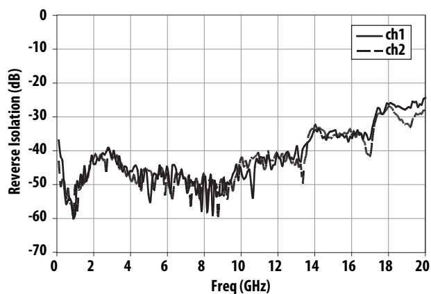
Figure 13. Isolation vs Frequency and channel
