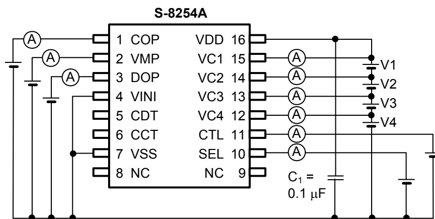
Figure 8 Test Circuit 5
