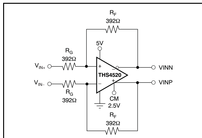
Figure 40. Basic Differential Input Signal Interface
