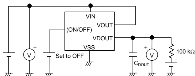
(c) Measurement circuit of the dynamic response for S-1701 Series D/E/F/K/L/M/U/V/W types
