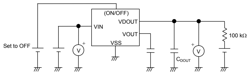
(b) Measurement circuit of the dynamic response for S-1701 Series A/B/C/G/H/J/X/Y/Z types
