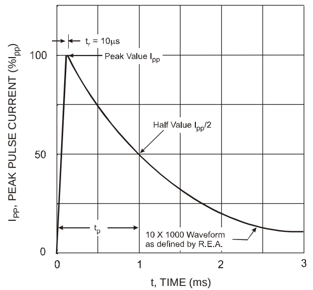
Fig. 4 Pulse Waveform
