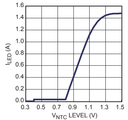
NTC Curve
