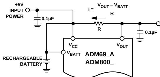
Figure 22. Rechargeable Battery
