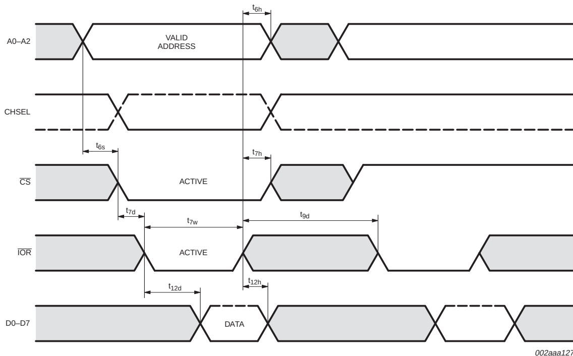
Fig 6. General read timing.
