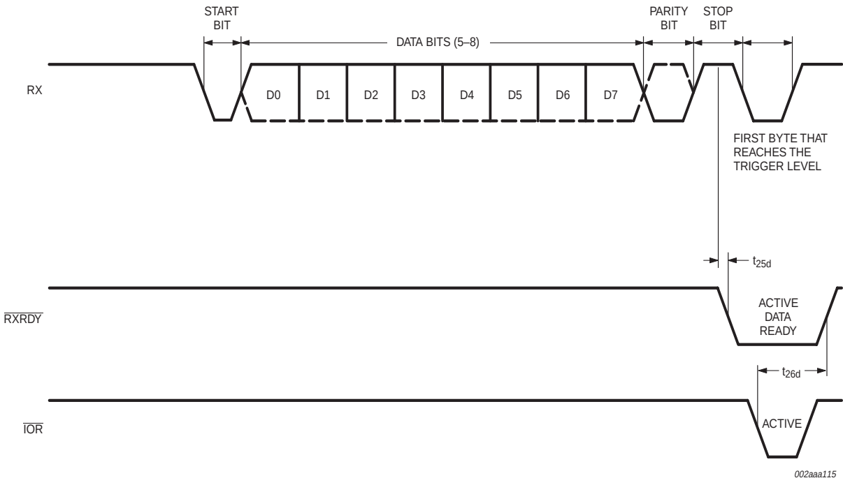
Fig 11. Receive ready timing in FIFO mode.
