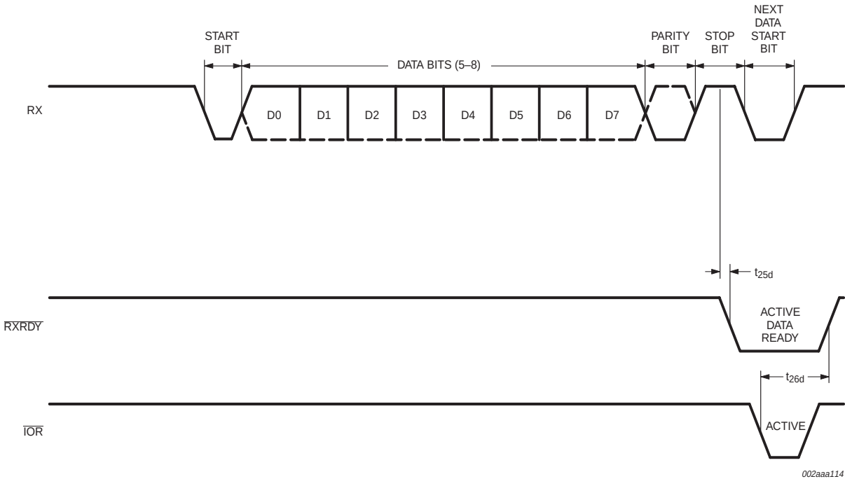
Fig 10. Receive ready timing in non-FIFO mode.
