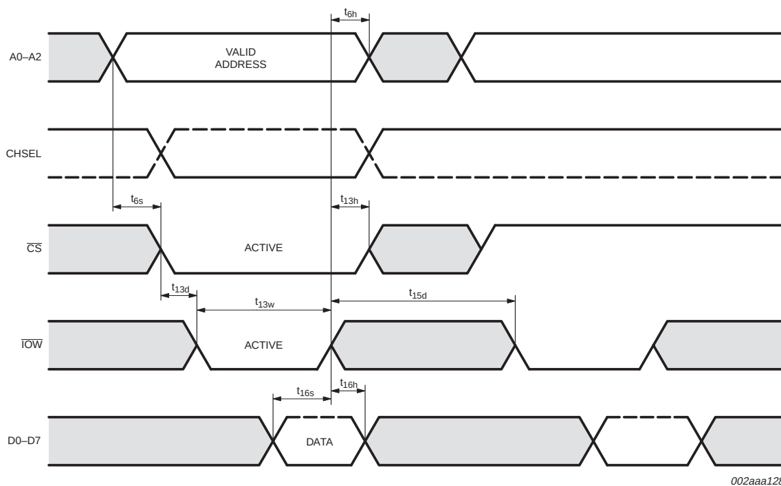
Fig 5. General write timing.
