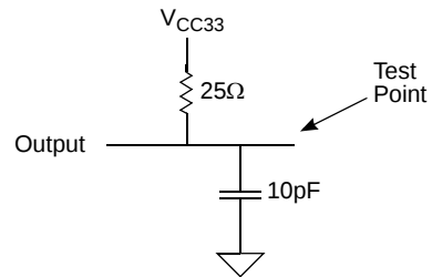
Figure 11: PCI T_{OV(max)} Falling Edge AC Test Load
