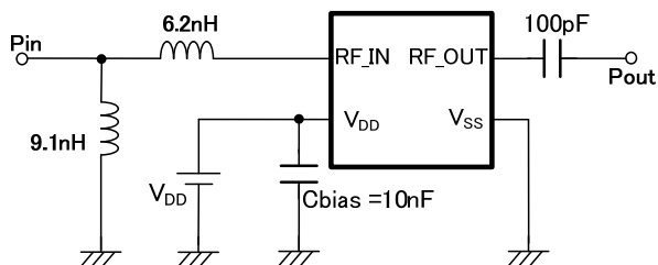
Figure 1: Fixed Bias
