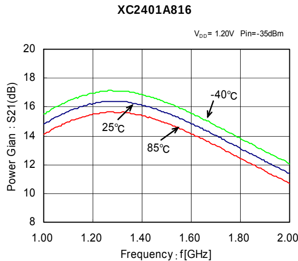
(17) Power Gain vs. Frequency
