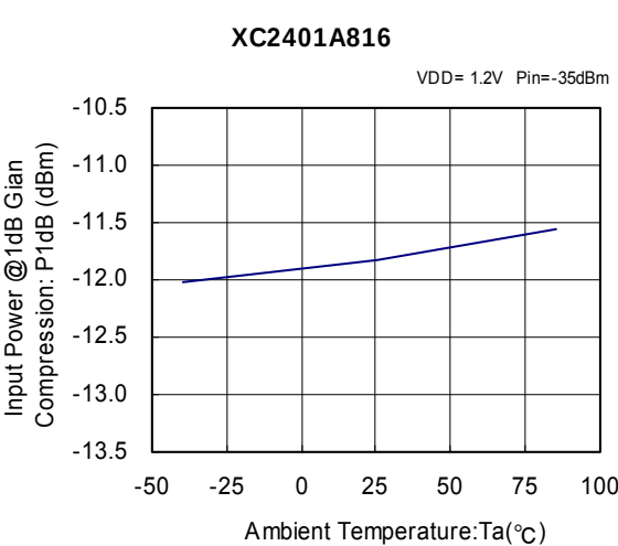
(16) Input Power @ 1dB Gain Compression vs. Ambient Temperature
