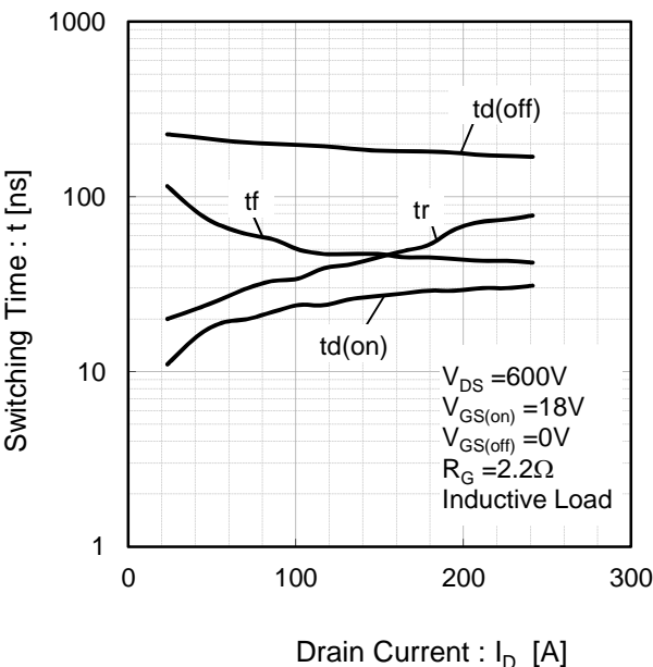
Fig.10 Switching Characteristics [ T_j=125^{\circ}\text{C} ]
