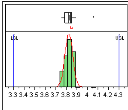
Figure 1. Vd Distribution@60mA.
