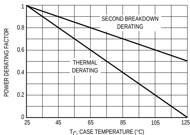
Figure 3. Power Derating
