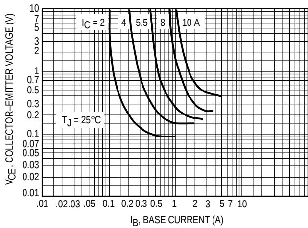
Figure 4. Typical Collector-Emitter Saturation Region
