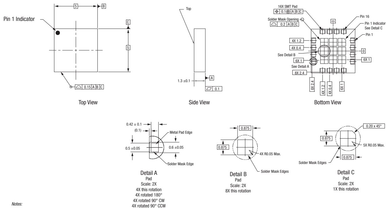
Figure 23. SKY66295-11 Package Dimensions
