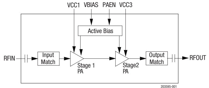
Figure 1. SKY66295-11 Block Diagram
